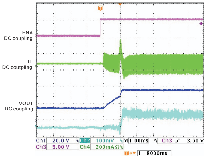
13. Start-up Waveform
