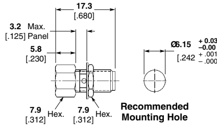
Part No. 1059733-1
