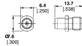
Part No. 1059716-1
