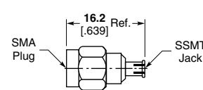
Part No. 1055697-1
