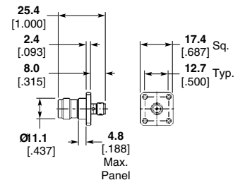
Part No. 1057841-1
