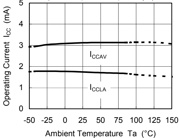
Operating Current vs. Temperature ( V^+=6V, R_T=33k\Omega, C_T=1000pF )
