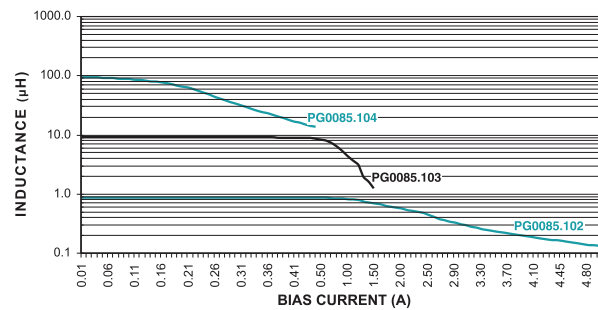
Inductance vs Current Characteristics
