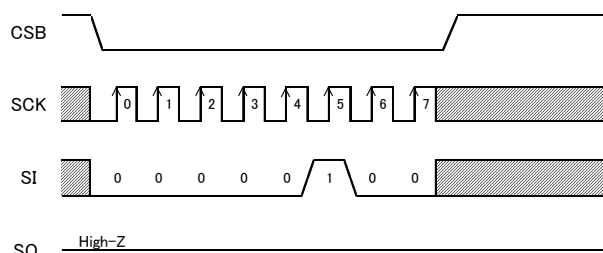
Figure 32. Write disable command
