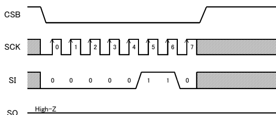
Figure 31. Write enable command
