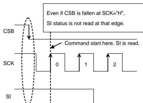
Figure 53. Operating timing
