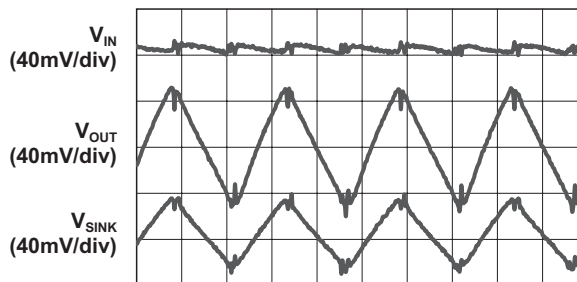
Load Characteristics ( V_{IN} = 3.2V ; 2X Mode; 27mA Load)
