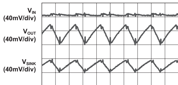
Load Characteristics ( V_{IN} = 4.1V ; 1.5X Mode; 27mA Load)
