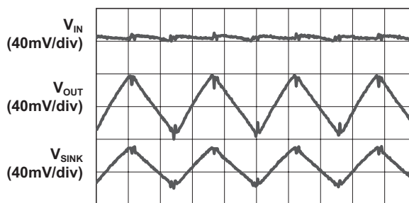
Load Characteristics ( V_{IN} = 2.8V ; 2X Mode; 18mA Load)
