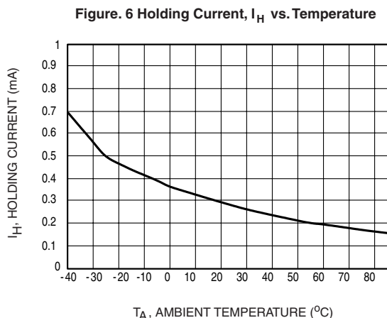
Figure 6 Holding Current, I_H vs. Temperature
