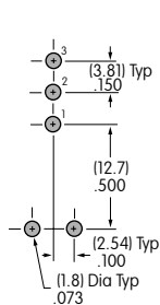
Single Pole
