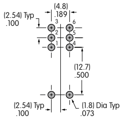
Double Pole
