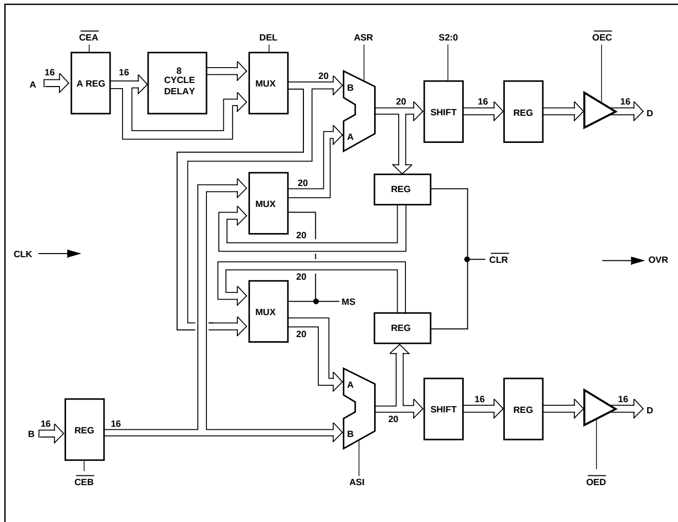
Fig. 3 Block diagram
