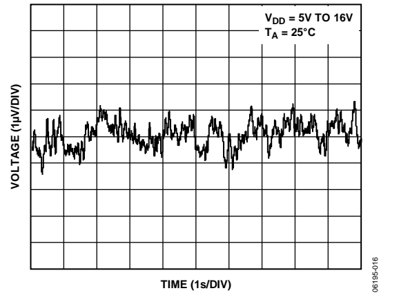
Figure 18. 0.1 Hz to 10 Hz Voltage Noise
