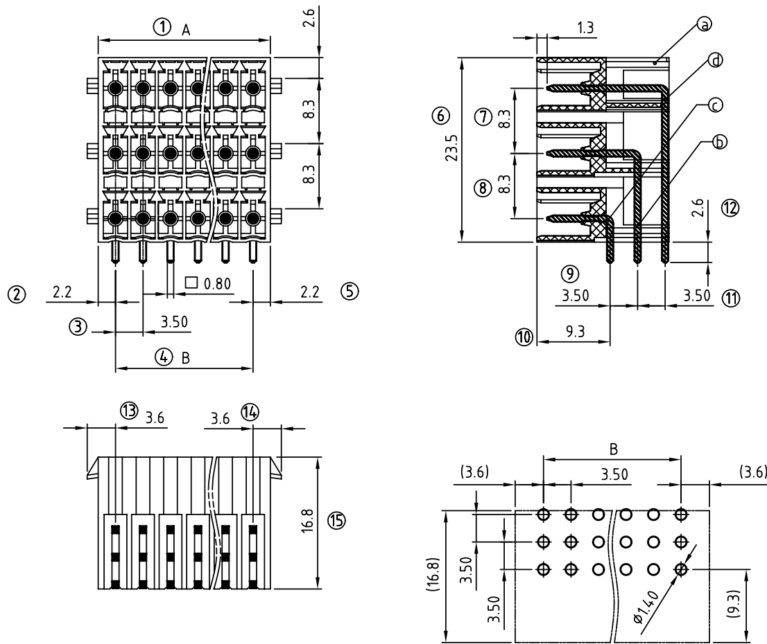
PCB Layout
