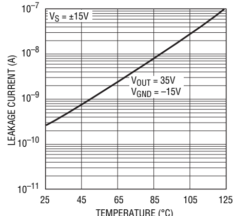
Output Leakage Current
