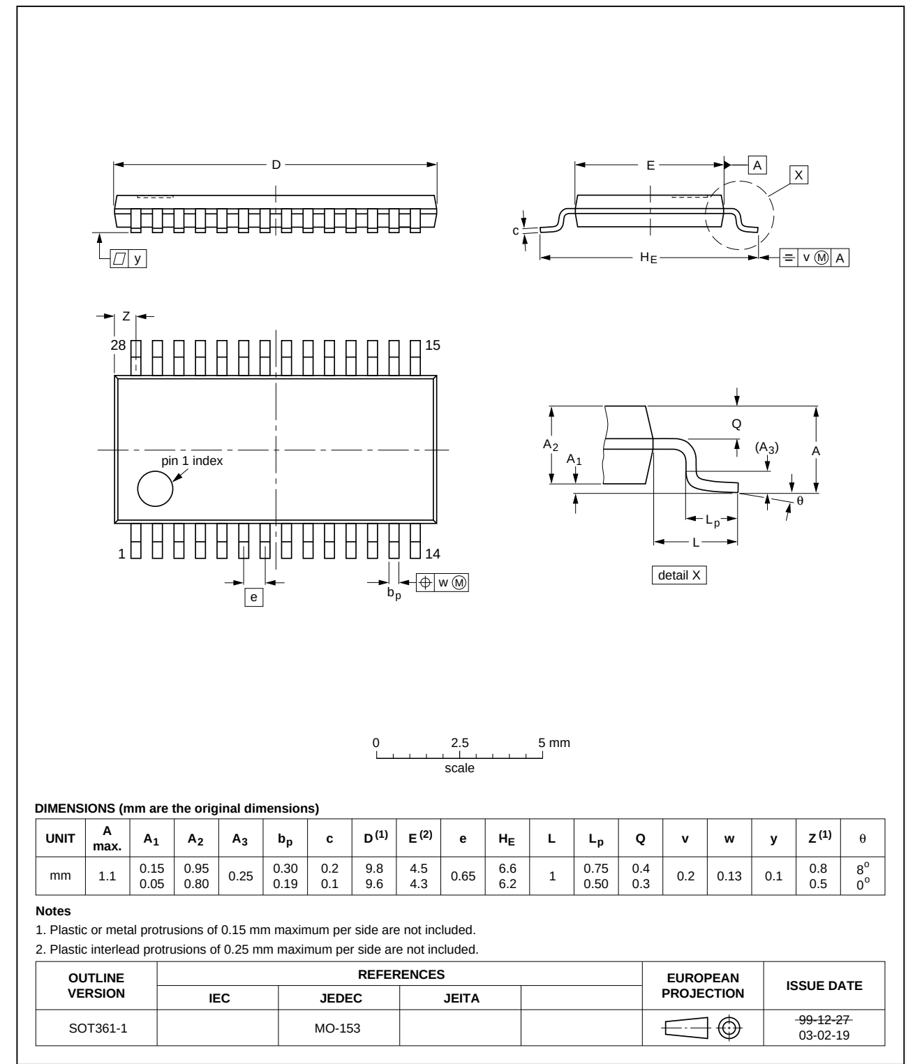
Fig 56. Package outline SOT361-1 (TSSOP28)
