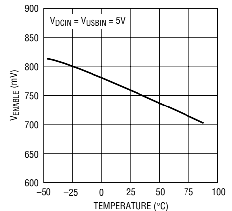
ENABLE Pin Threshold (On-to-Off) vs Temperature
