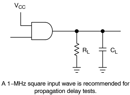
Figure 4. Test Circuit
