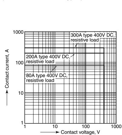
2.-(2) Max. value for switching capacity (80A, 200A and 300A types)
