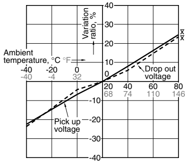
1.-(1) Ambient temperature characteristics (10A type)
