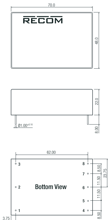
Dimension Drawing (mm)
