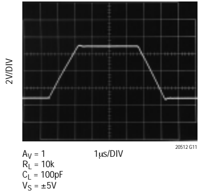
Transient Response
