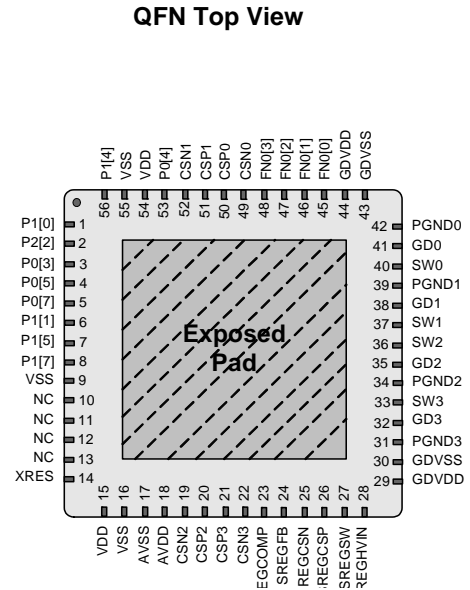
Figure 12-1. CY8CLED04D0x 56-Pin PowerPSoC Device
