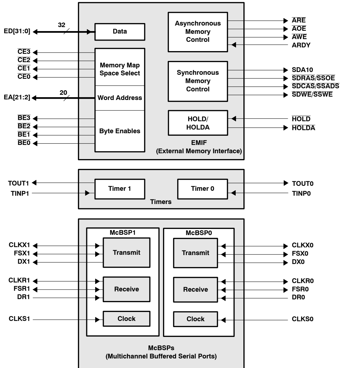
Figure 3. Peripheral Signals
