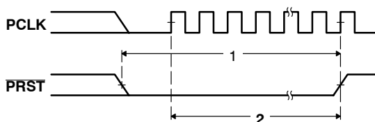
Figure 31. PCI Reset ( \overline{PRST} ) Timings
