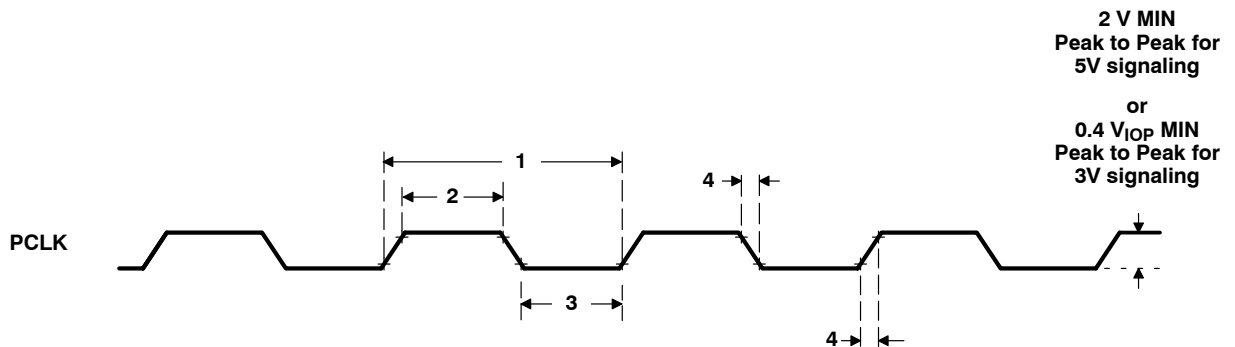
Figure 13. PCLK Timings
