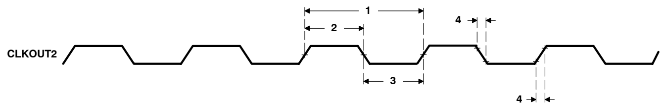
Figure 14. CLKOUT2 Timings
