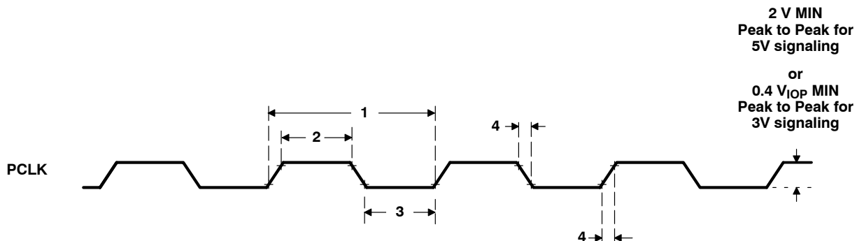
Figure 13. PCLK Timings
