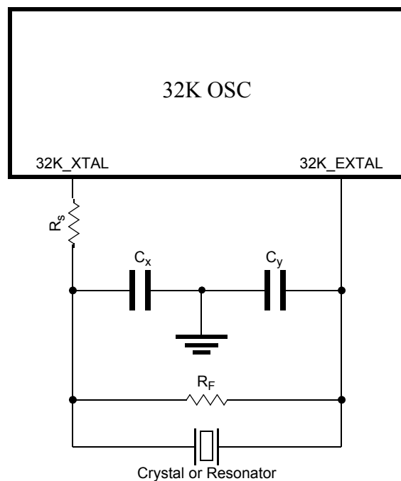
Figure 1-3. 32K OSC Crystal/Resonator Connection
