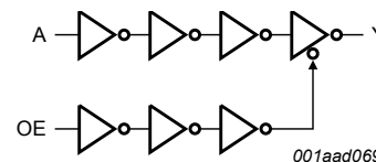
Figure 3. Logic diagram
