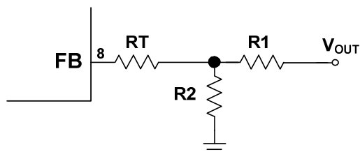
Figure 4: T-Type Network
