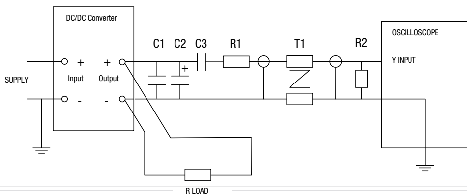
NDS 24V Input, Single Output
