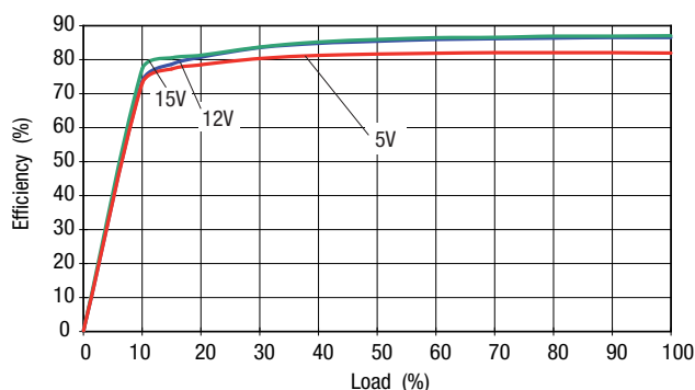
NDS 24V Input, Dual Output
