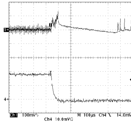
PWM to PSM 5 V Converter ( V_{IN} = 10 V )
