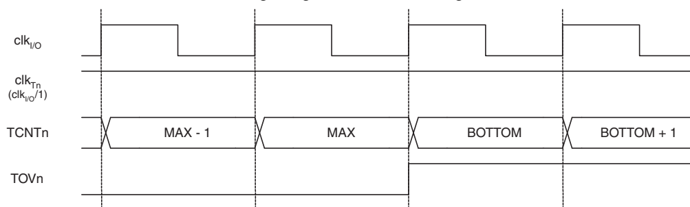
Figure 4-33. Timer/Counter Timing Diagram, no Prescaling
