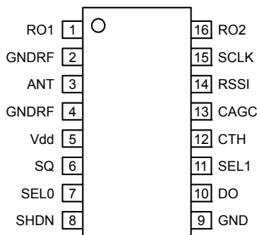
MICRF219YQS
