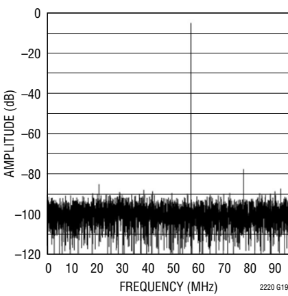
LTC2220-1: 8192 Point FFT, f_{IN} = 500\text{MHz} , -6dB, 1V Range, LVDS Mode
