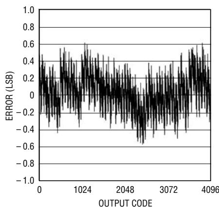
LTC2220-1: INL, 2V Range
