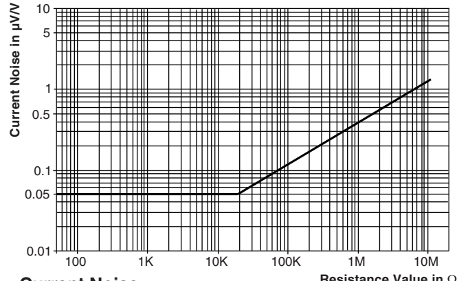
Current Noise
