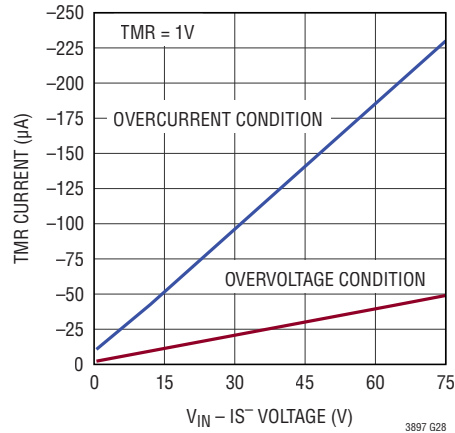
TMR Current vs V_{IN} - IS^{-} Voltage
