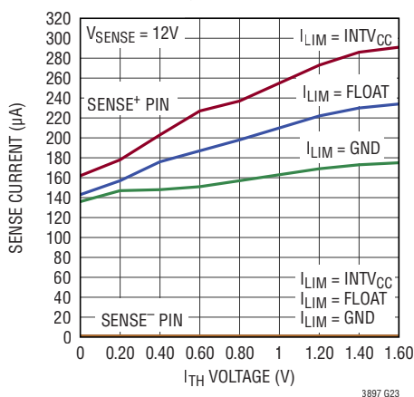
SENSE Pin Input Current vs I_{TH} Voltage
