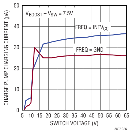
BOOST-SW Charge Pump Charging Current vs Switch Voltage
