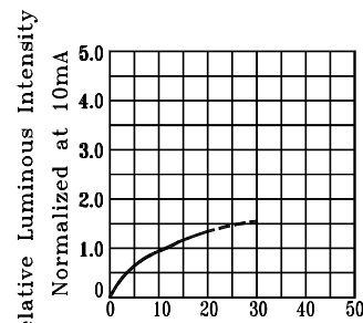
Fig.4 Relative Luminous Intensity
