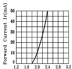
Fig.2 Forward Current vs.
