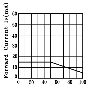
Fig.3 Forward Current
