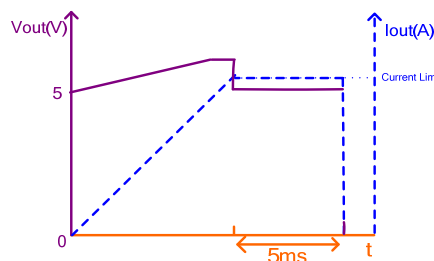
Figure 7: Over-Current Limit
