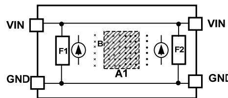
Figure 5: EMI Reduction
