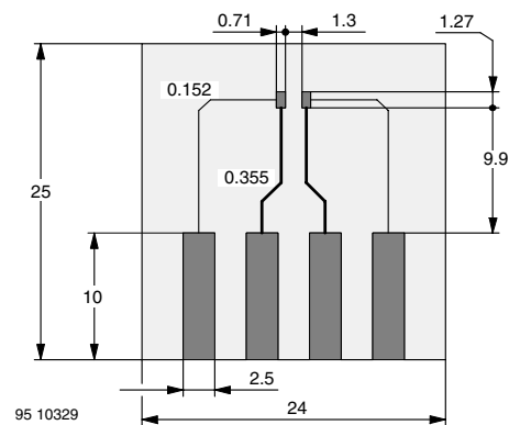
Figure 4. Board for R_{thJA} definition (in mm)
