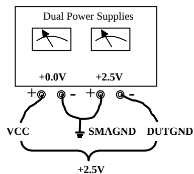
Offset / “Split” Power Supply Configuration
