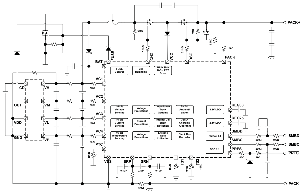
Figure 1. bq30z554-R1 Implementation
