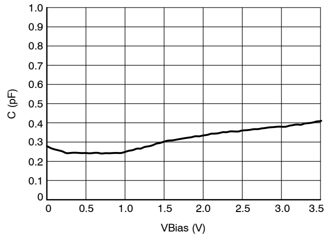
Figure 11. CV Characteristics
