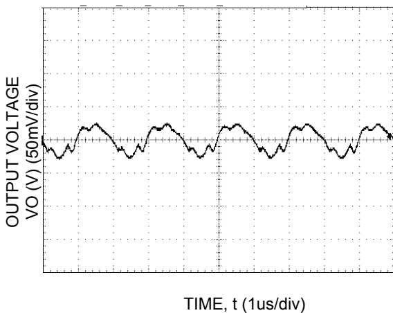
Fig-21. Typical output ripple and noise ( C_O=2x47\mu F ceramic, V_{IN} = 12V , I_O = I_{O,max} ).
