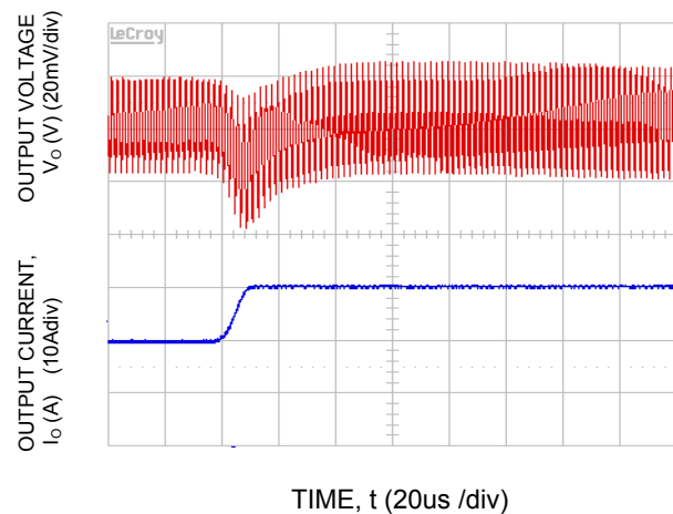
Fig-40. Transient Response to Dynamic Load Change from 50% to 100% at 12V in , C out = 1x47uF +5x330uF, C T tune=10nF & R T tune=178 ohms
