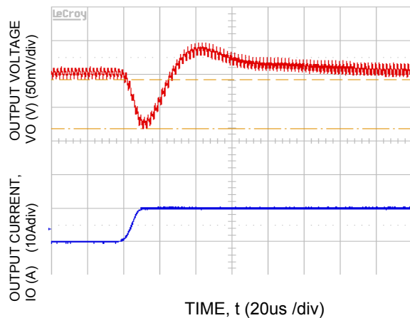
Fig-22. Transient Response to Dynamic Load Change from 50% to 100% at 12Vin, C_{out}= 5x47\mu F + 1x330\mu F , C_{Tune}=2200pF & R_{Tune}=220 ohms
