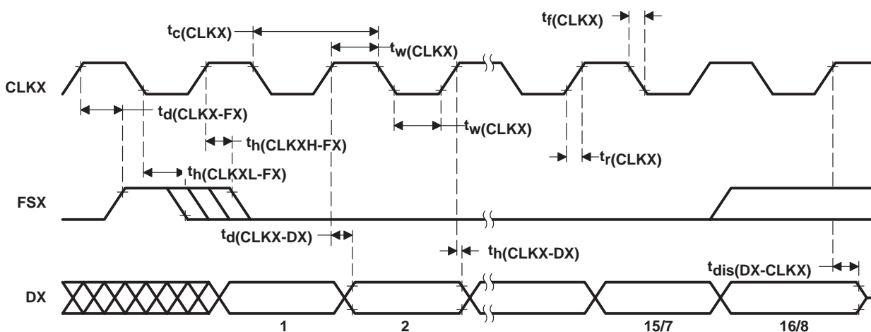
Figure 18. Serial-Port Transmit Timing of External Clocks and External Frames for 'C203/LC203
