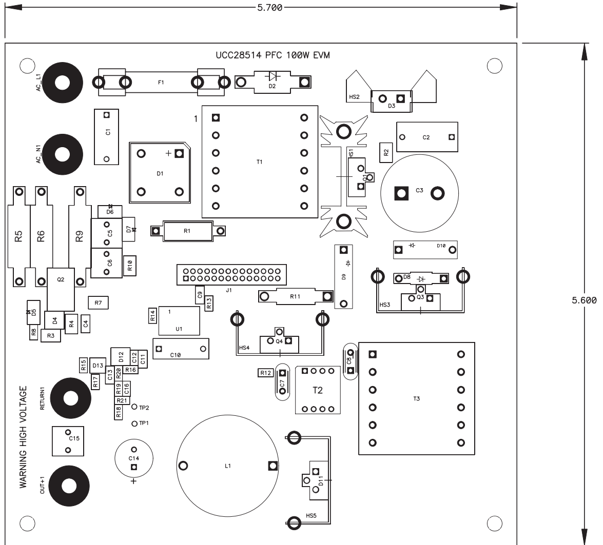
Figure 4. Mother Board HPA013
