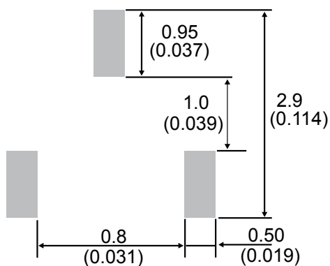
Figure 11. SOT323-3L recommended footprint
