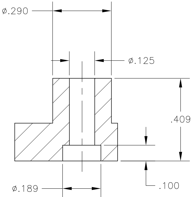
DETAIL A BOTH ENDS
