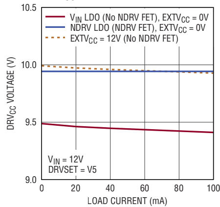
DRV CC vs Load Current
