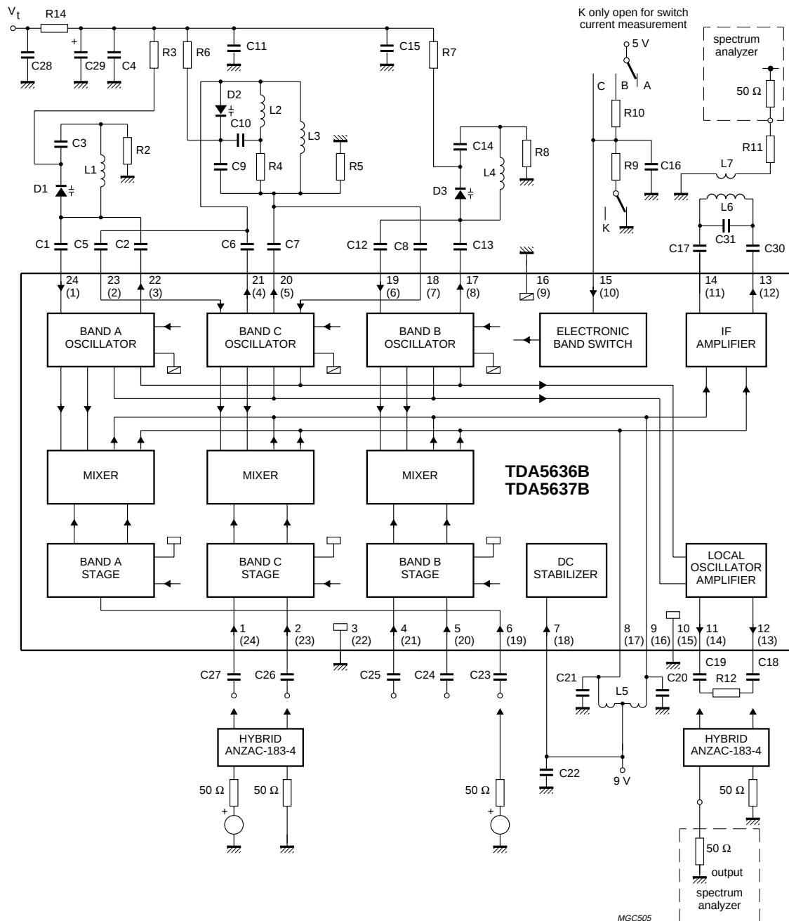
Fig.17 Measurement and application circuit.
