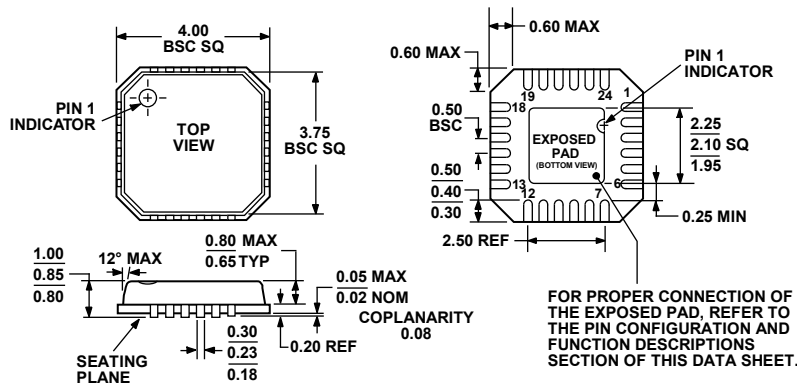
COMPLIANT TO JEDEC STANDARDS MO-220-VGGD-2 Figure 69. 24-Lead Lead Frame Chip Scale Package [LFCSP_VQ] 4 mm x 4 mm Body, Very Thin Quad (CP-24-1) Dimensions shown in millimeters
