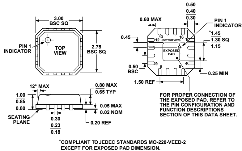
Figure 68. 16-Lead Lead Frame Chip Scale Package [LFCSP_VQ] 3 mm x 3 mm Body, Very Thin Quad (CP-16-2) Dimensions shown in millimeters
