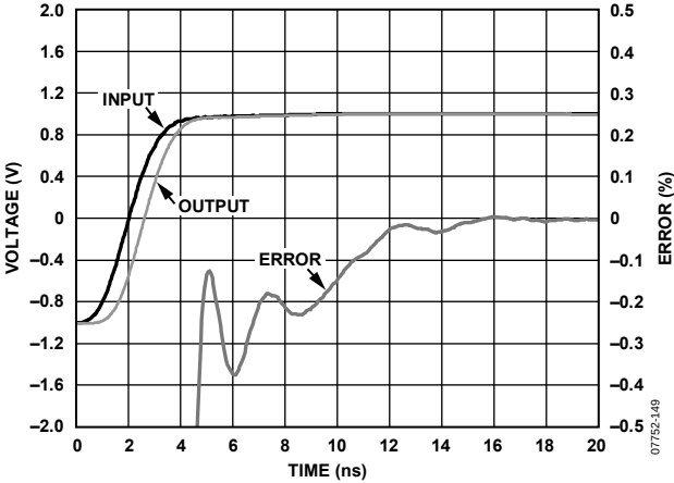
Figure 49. Settling Time
